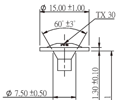
Tellerkopf
