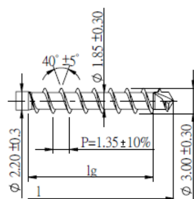
Quickdrill DP+
