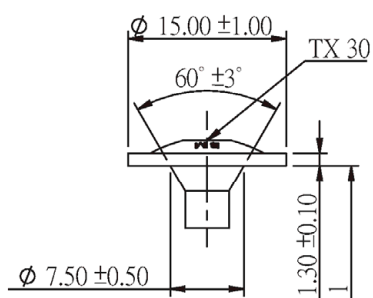
Tellerkopf
