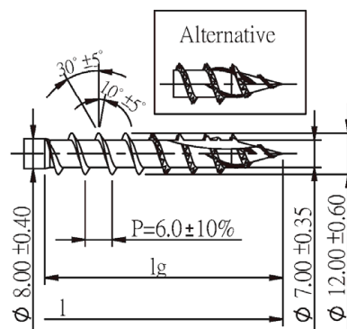
Quickdrill III
