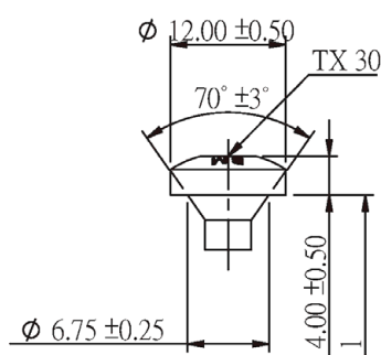
Pan Head
