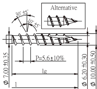
Quickdrill II
