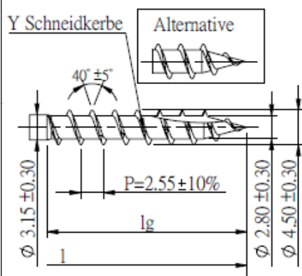
Quickdrill
