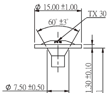
Tellerkopf
