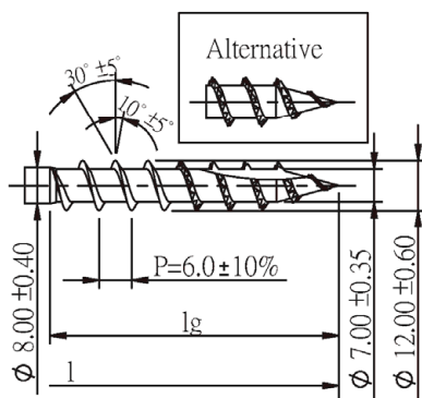
Quickdrill II
