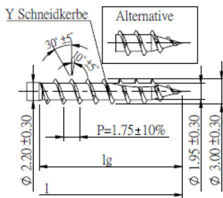
Quickdrill +
